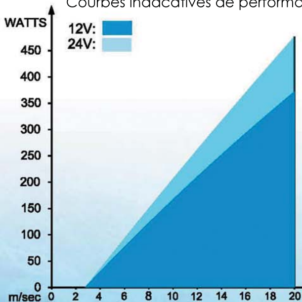
Courbes indicatives de performances
