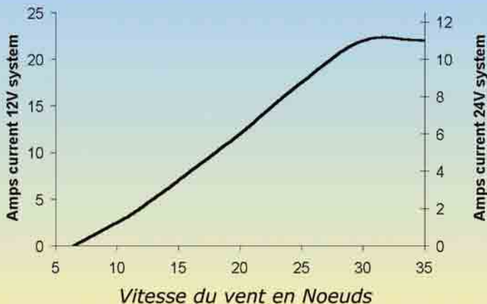
Performances mode Eolienne
